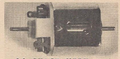
26 GAUGE WIRE - BAL. AND EPOXIED ARCO MAGNETS
